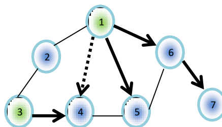
Fig 3. Reactive AODV
